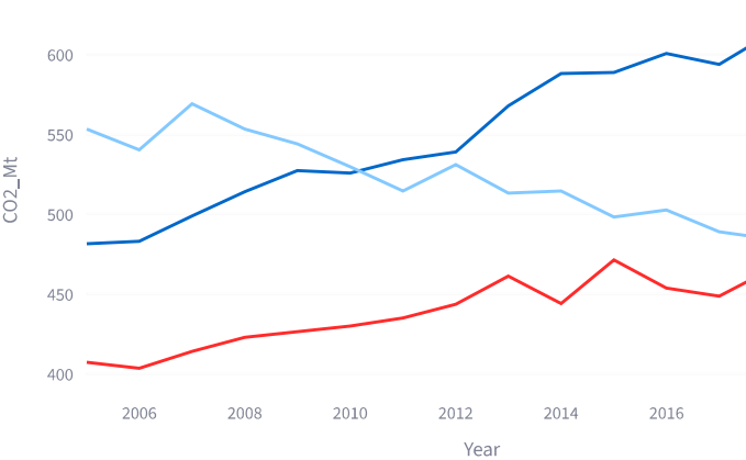
Total CO2 (Mt) Over Time
